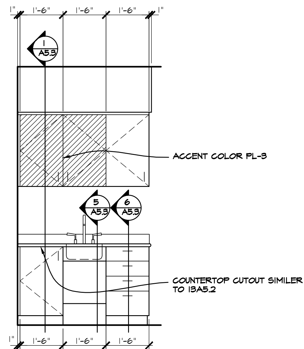
10 ELEVATION EXAM SJ 158 1/2" = 1'-0"
