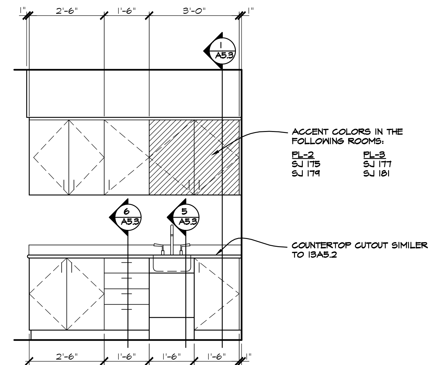
11 ELEVATION EXAM SJ 175-177-179-181 1/2" = 1'-0"
