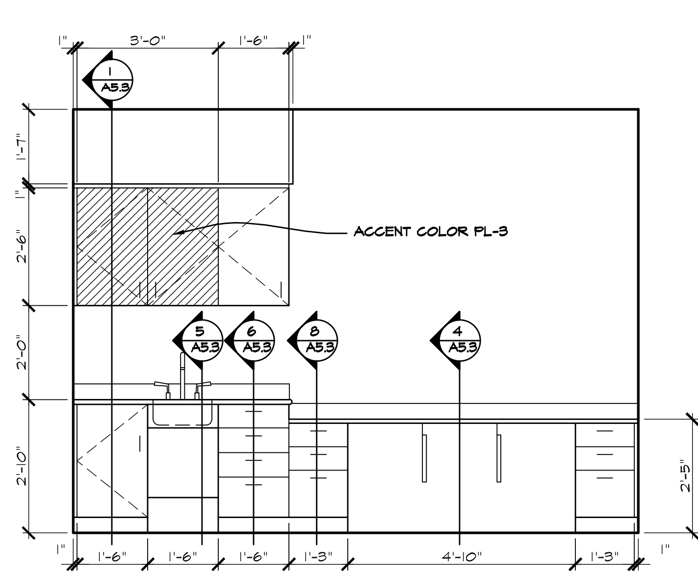
8 ELEVATION INTAKE SJ 154 1/2" = 1'-0"
