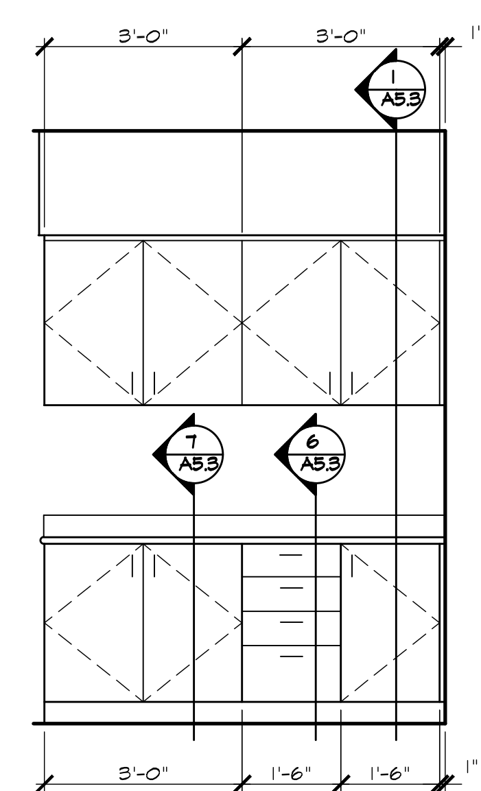
20 ELEVATION CONFERENCE ROOM SJ 182 1/2" = 1'-0"
