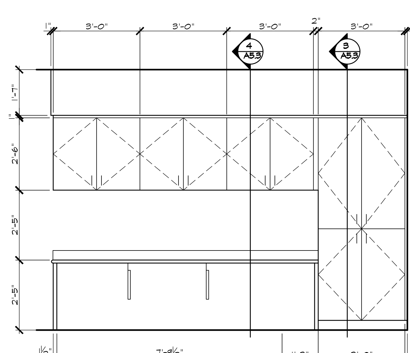
16 ELEVATION AUDIOLOGY SJ 169 1/2" = 1'-0"
