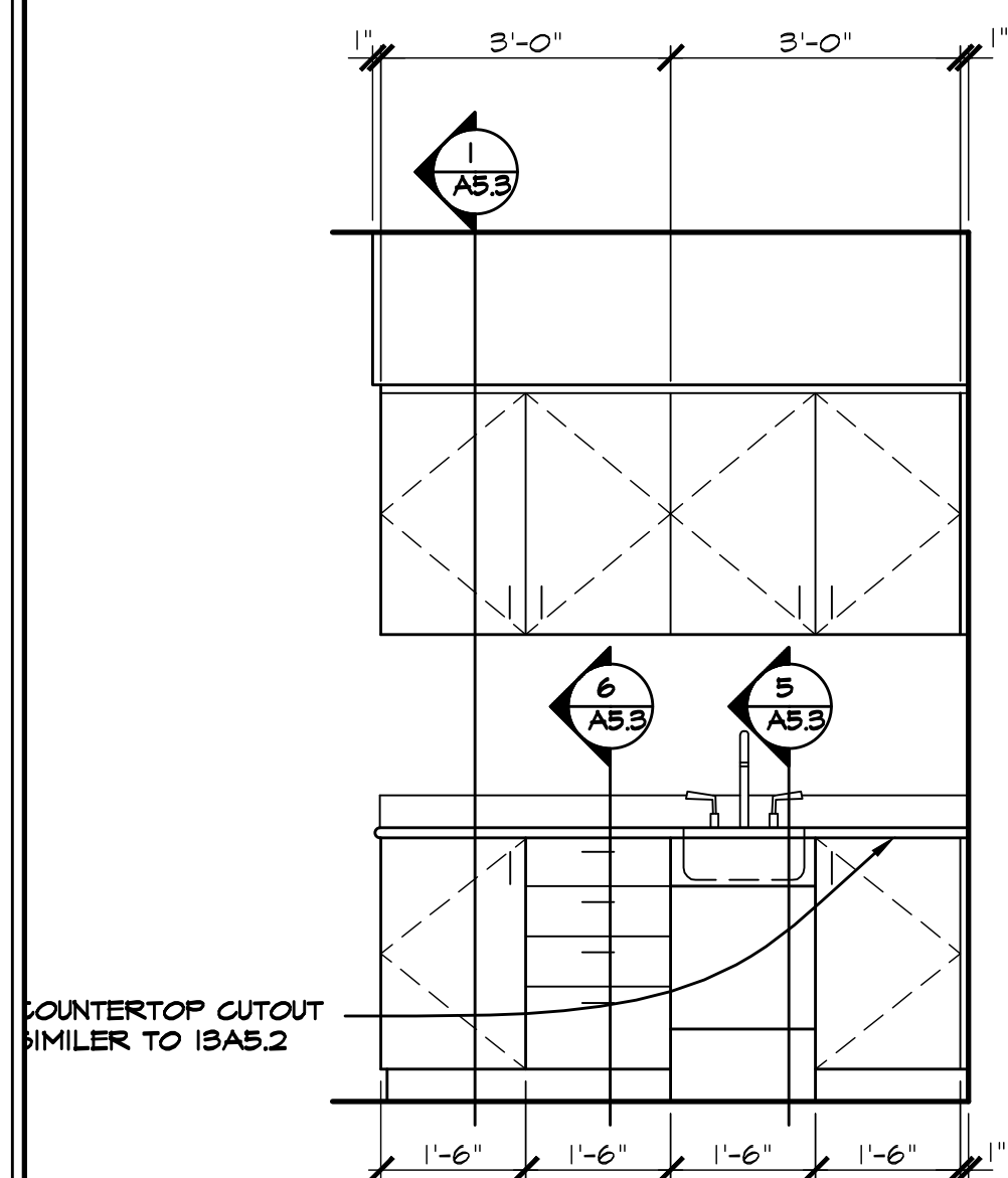
12 ELEVATION PROCEDURE SJ 168 1/2" = 1'-0"
