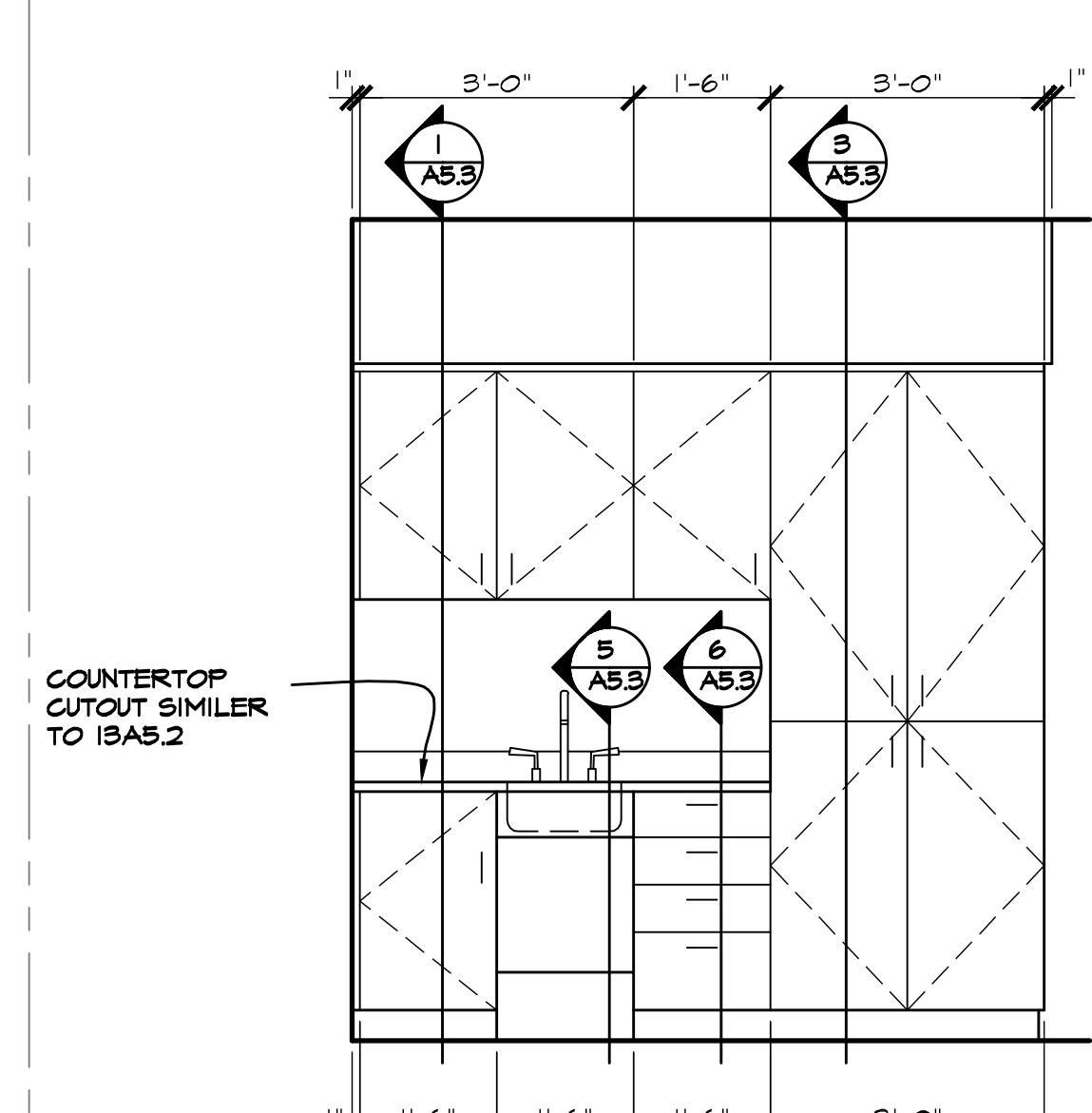
17 ELEVATION ULTRASOUND SJ 177 1/2" = 1'-0"
