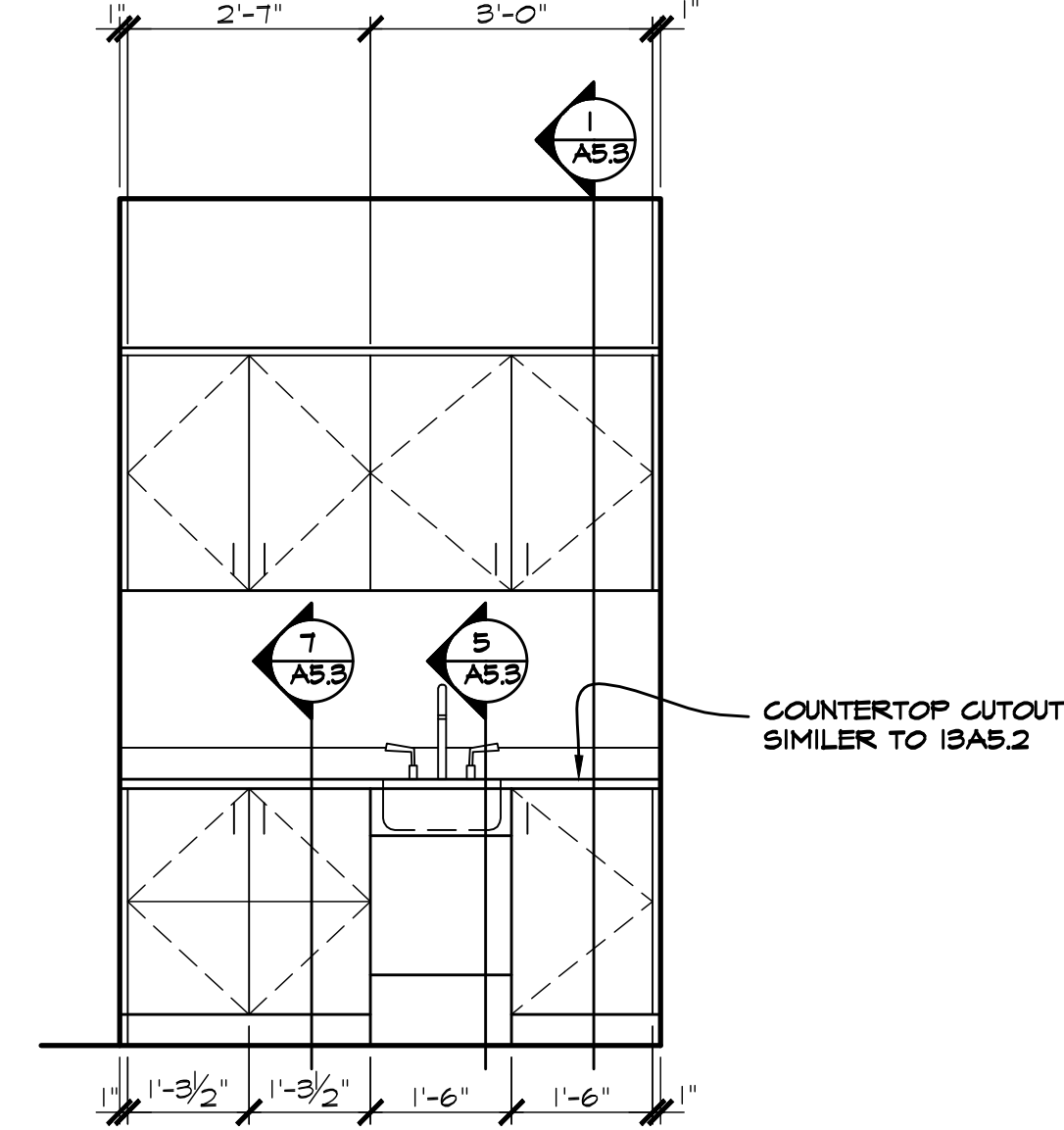
21 ELEVATION UTILITY SJ 166 1/2" = 1'-0"
