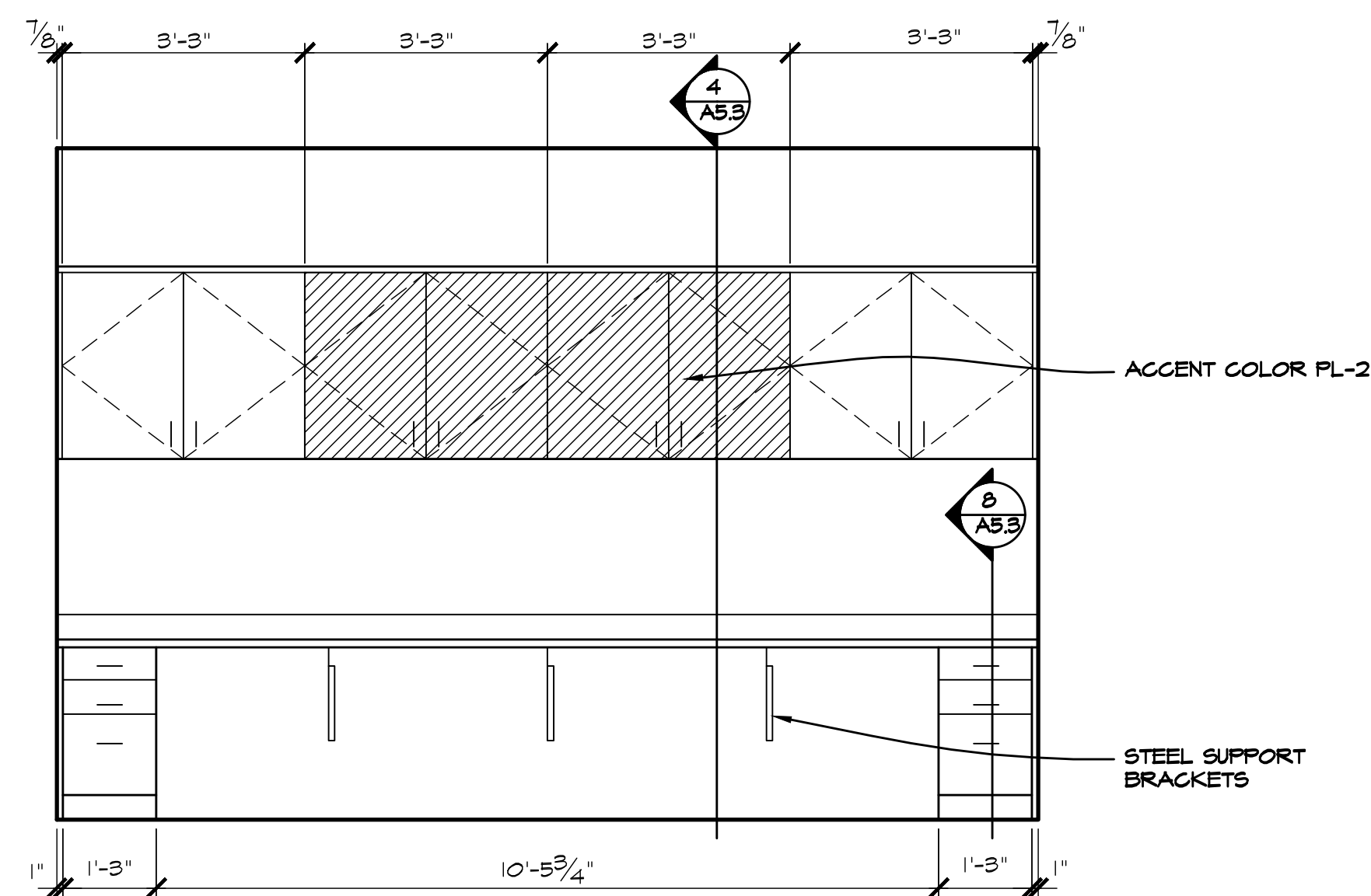
19 ELEVATION NURSE WORK ROOM SJ 163 1/2" = 1'-0"
