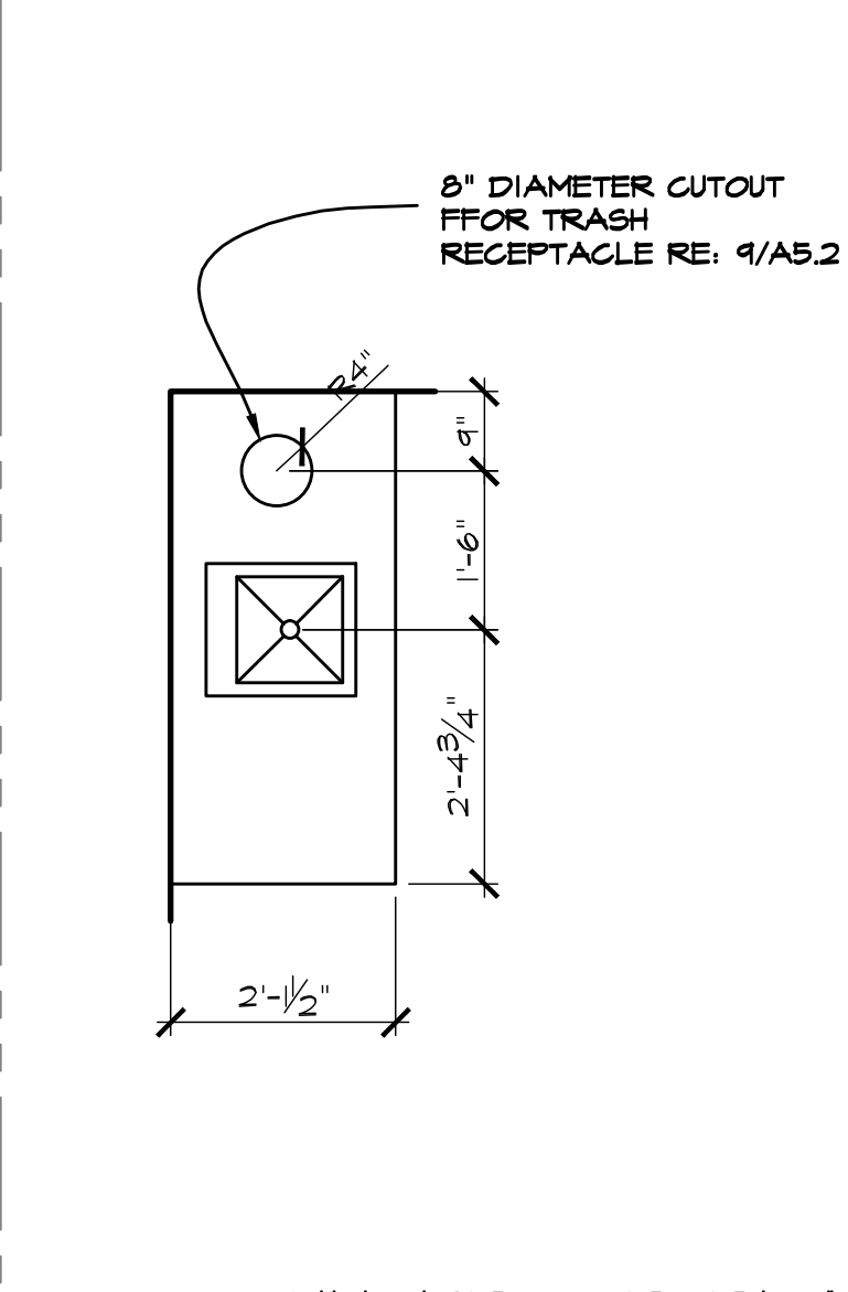
13 COUNTERTOP PLAN TYPICAL EXAM ROOM 1/2" = 1'-0"
